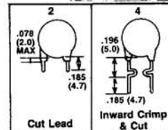
Alternate Lead Configurations Available in Production Quantities
